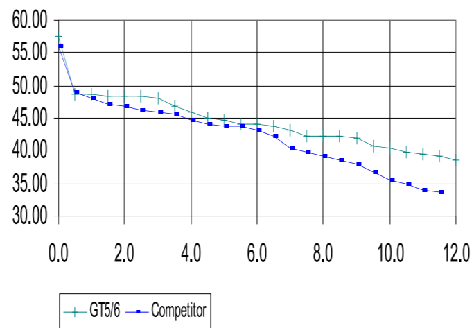
BULB PERFORMANCE
