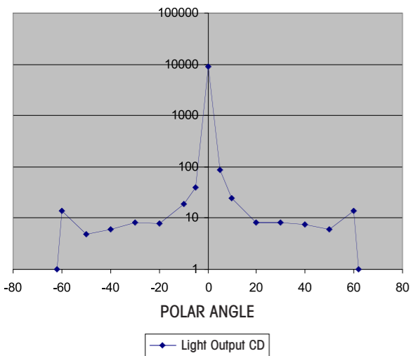
LIGHT OUTPUT GT CAPLAMP
